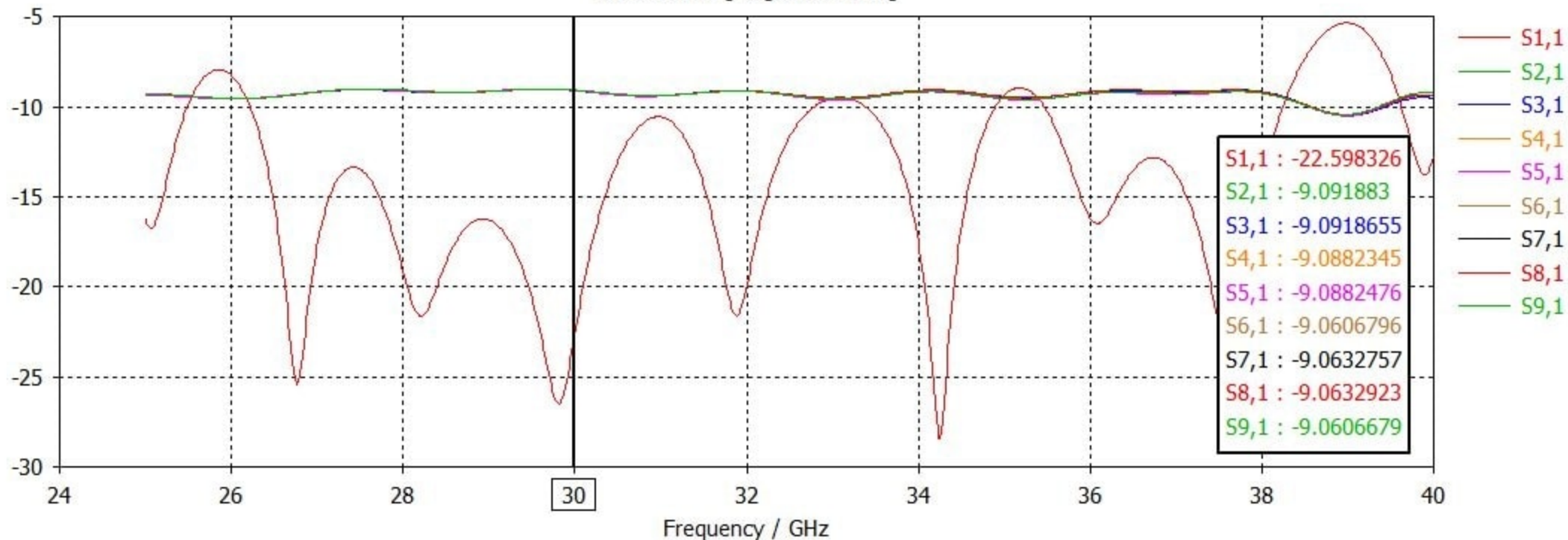
S-Parameter [Magnitude in dB]
