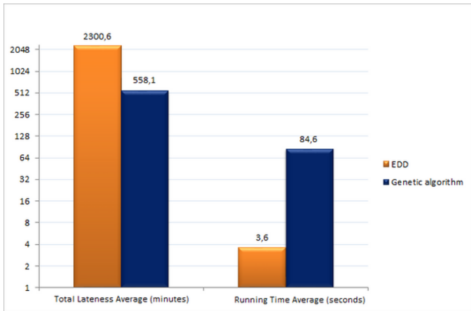
Figure 1. Comparison of Running Time Average and Total Lateness Average between Genetic Algorithm and EDD.
