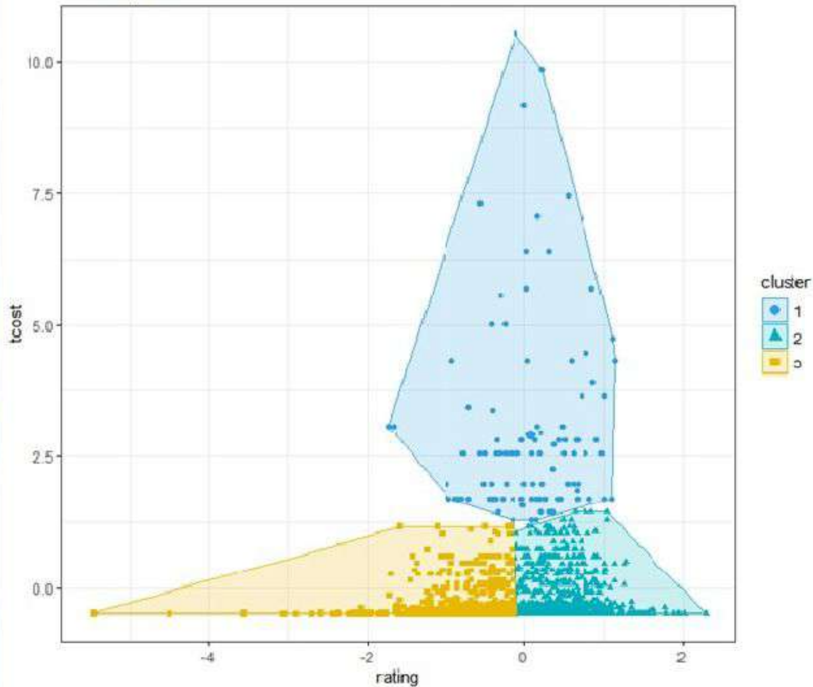
Cluster plot
