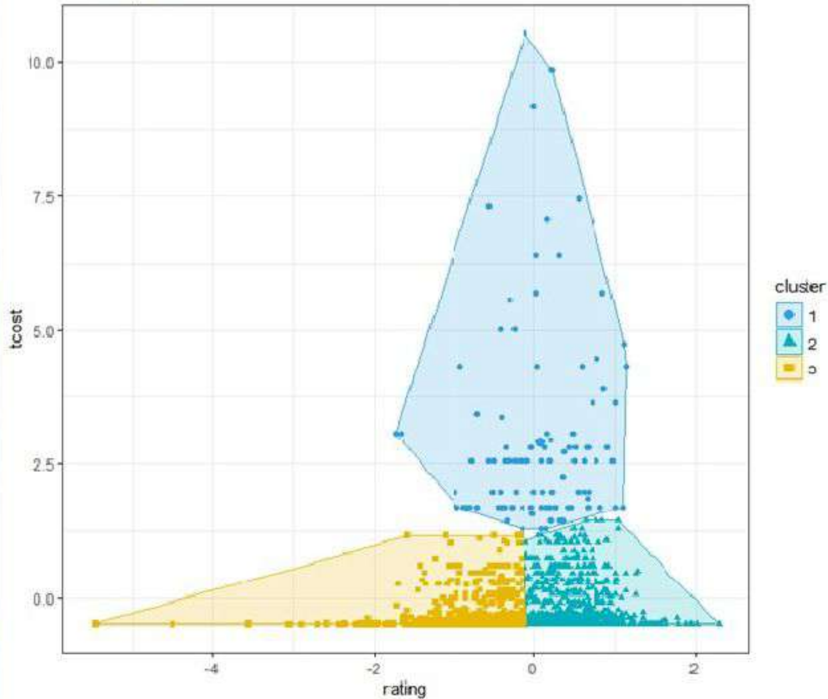
Cluster plot
