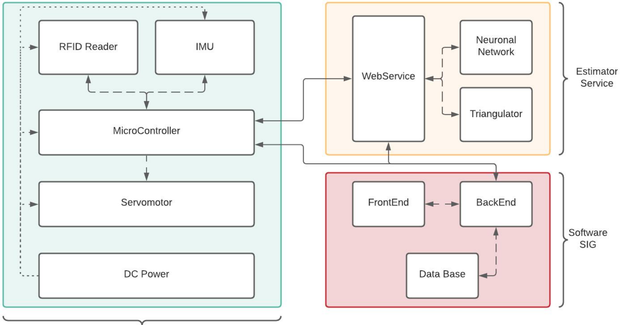
Radar System
